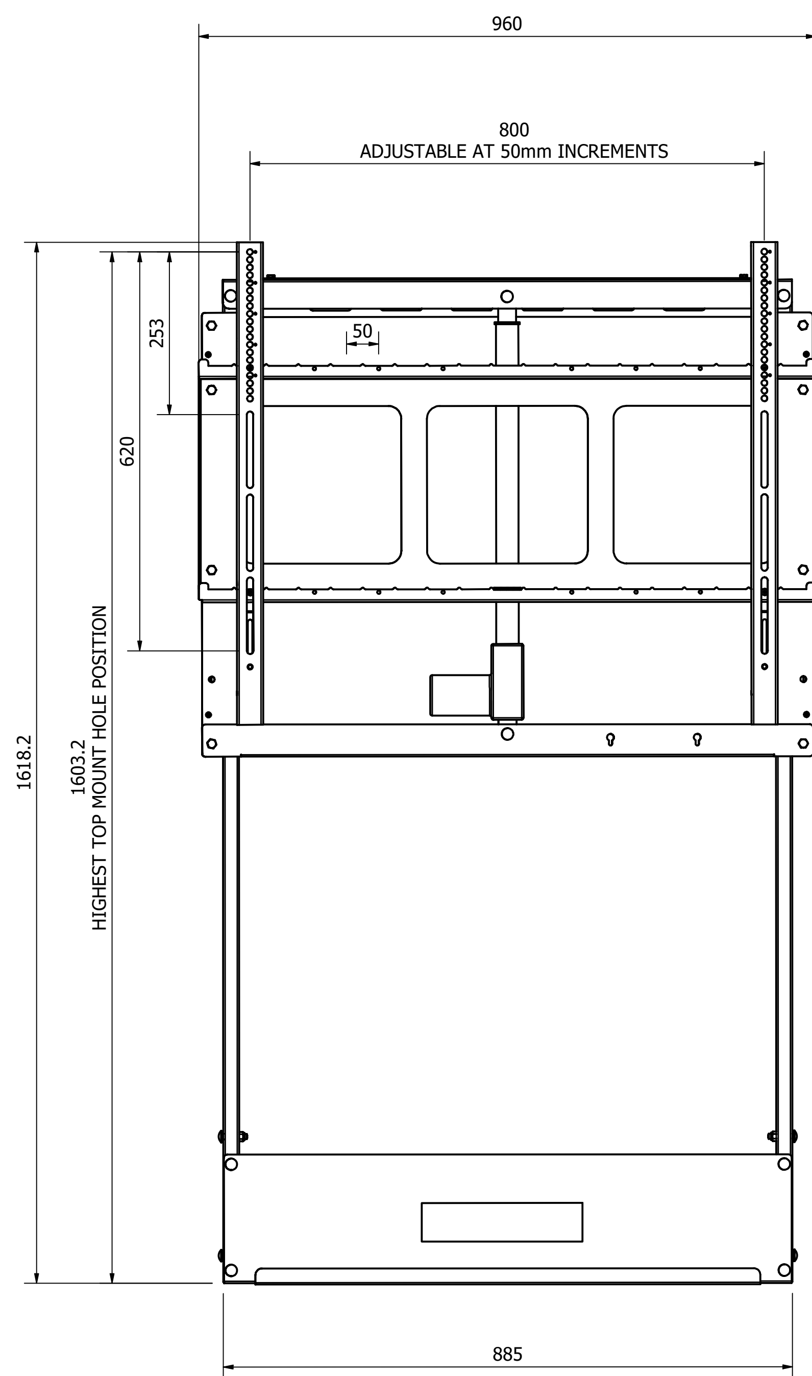
FRONT VIEW TOP POSITION
